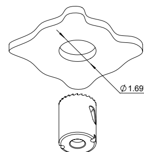
Ceiling Cut-Out: Ø1.69" Fixture Dimensions
