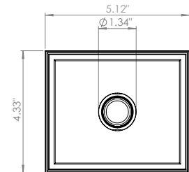
Ceiling Cut-Out: 4.49" x 5.28" Fixture Dimensions
