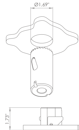
Ceiling Cut-Out: Ø1.69" Fixture Dimensions
