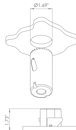
Ceiling Cut-Out: Ø1.69" Fixture Dimensions
