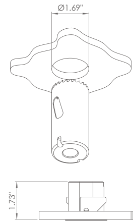
Ceiling Cut-Out: Ø1.69" Fixture Dimensions
