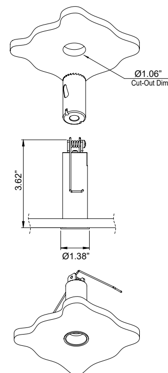
Ceiling Cut-Out: Ø1.06" Fixture Dimensions
