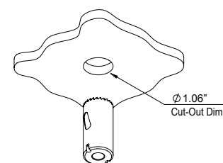
Ceiling Cut-Out: Ø1.06" Fixture Dimensions
