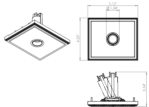
Fixture Dimensions
