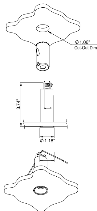
Fixture Dimensions
