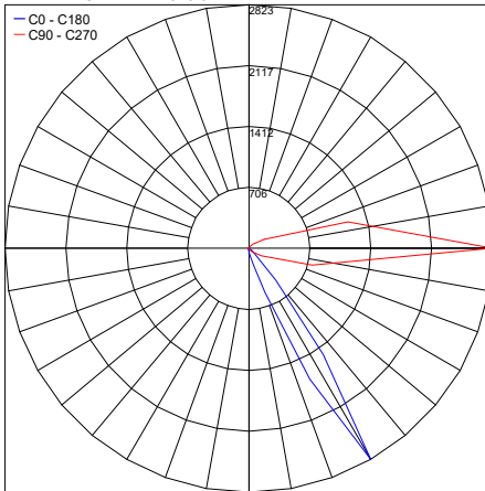
PHOTOMETRIC FILENAME : 200CENT W30 WALLWASH 30° 3W 12° IES
