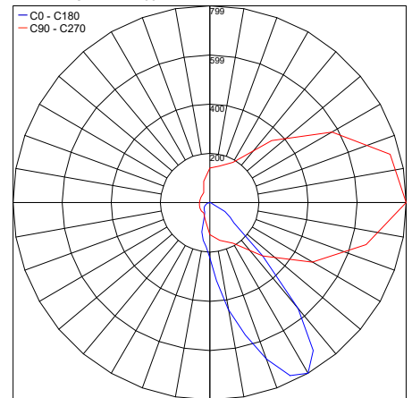
PHOTOMETRIC FILENAME : 200CENT W30 WALLWASH 30° 6.2W 36° IES
