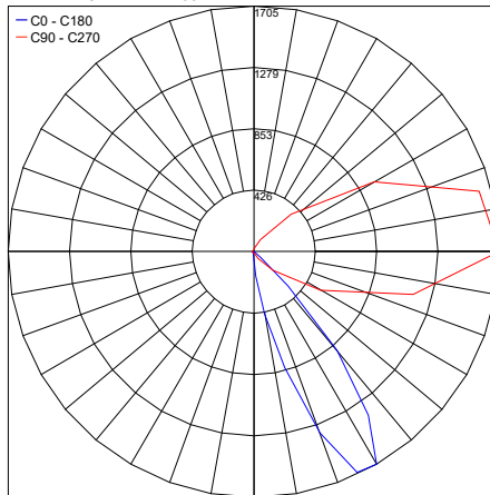
PHOTOMETRIC FILENAME : 200CENT W30 WALLWASH 30° 5.9W 24° IES
