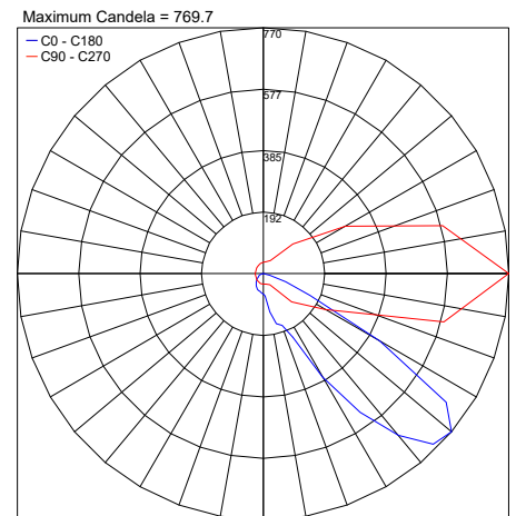
PHOTOMETRIC FILENAME : 200CENT W50 WALLWASH 50° 6.2W 36".IES
