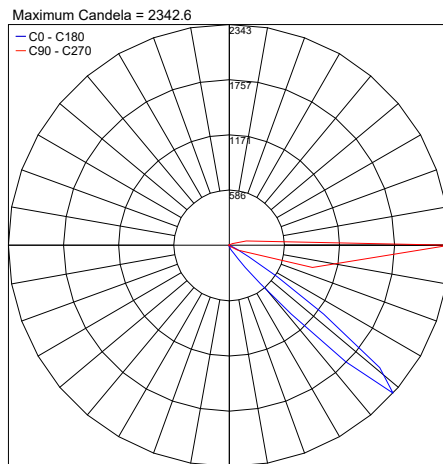
PHOTOMETRIC FILENAME : 200CENT W50 WALLWASH 50° 3W 12".IES
