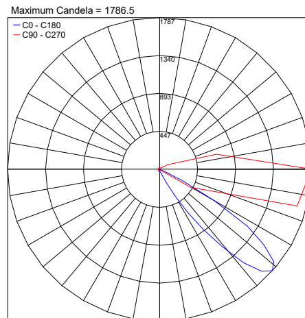
PHOTOMETRIC FILENAME : 200CENT W50 WALLWASH 50° 5.9W 24".IES
