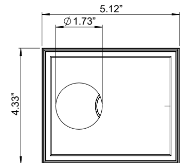
Ceiling Cut-Out: 4.49" x 5.28" Fixture Dimensions
