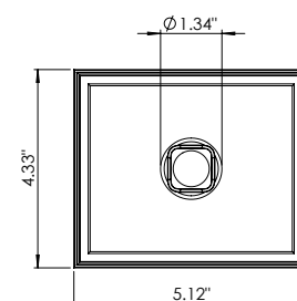
Ceiling Cut-Out: 4.49" x 5.28" Fixture Dimensions
