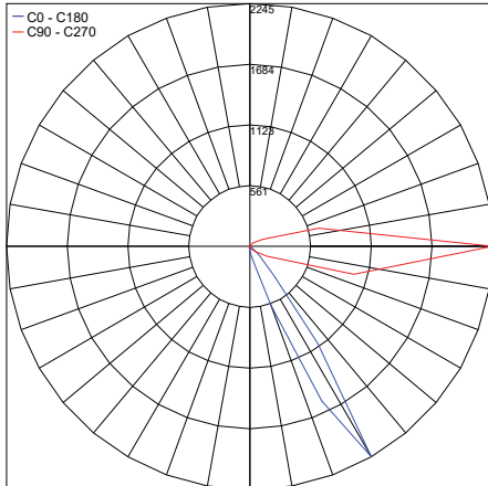
PHOTOMETRIC FILENAME : 200CENT WALLWASH30-SEMI-250LM-12".IES
