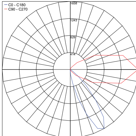
PHOTOMETRIC FILENAME : 200CENT WALLWASH30-SEMI-500LM-24".IES
