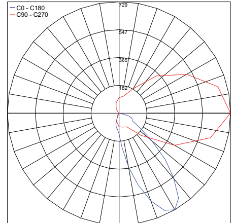
PHOTOMETRIC FILENAME : 200CENT WALLWASH30-SEMI-750LM-36".IES
