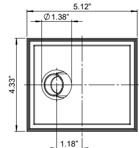
Ceiling Cut-Out: 4.49" x 5.28" Fixture Dimensions
