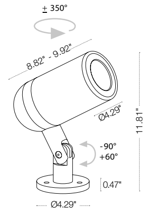
Fixture Dimensions
