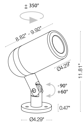
Fixture Dimensions
