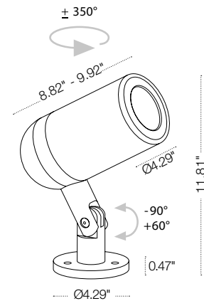
Fixture Dimensions
