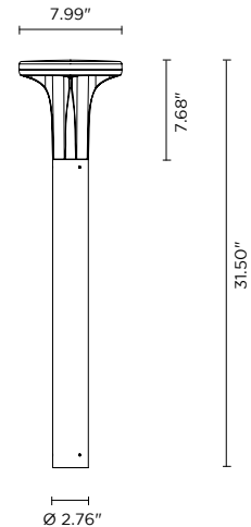
Fixture Dimensions:
