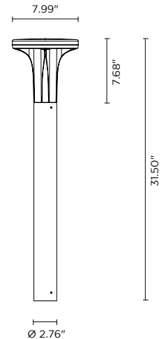
Fixture Dimensions:
