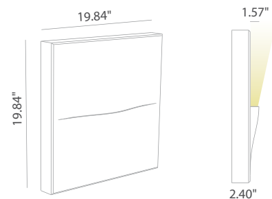
Wall Cut-Out: 20.08" x 20.08" Fixture Dimensions
