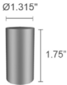
PPMP03159 Core Drilled Application Sleeve
