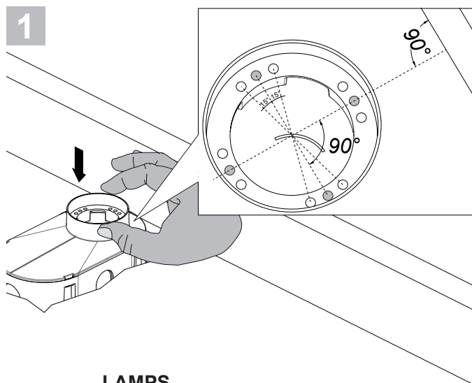
LAMPS ALIGNMENT
