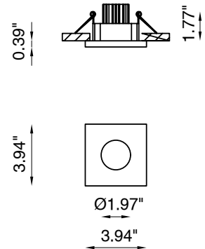
Fixture Dimensions
