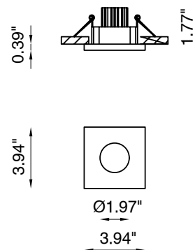
Fixture Dimensions
