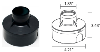
WC1501 Outer Casing For in-grade use
