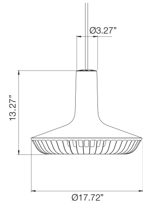
Fixture Dimensions
