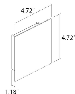
Fixture Dimensions
