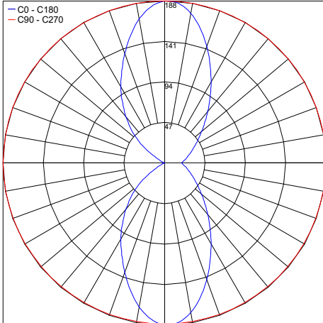
PHOTOMETRIC FILENAME : BERICA 3.0 K 59°X90° [3000K 8W].IES
