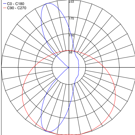
PHOTOMETRIC FILENAME : BERICA 3.0 A [3000K 8W].IES
