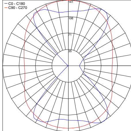
PHOTOMETRIC FILENAME : BERICA 3.0 D [3000K 8W].IES
