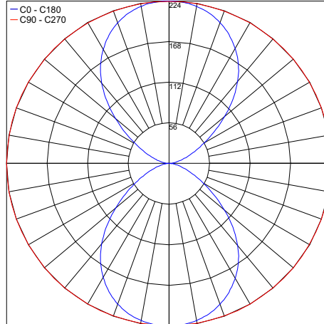
PHOTOMETRIC FILENAME : BERICA 3.0 L 45°X96° [3000K 8W].IES
