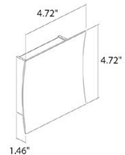
Fixture Dimensions
