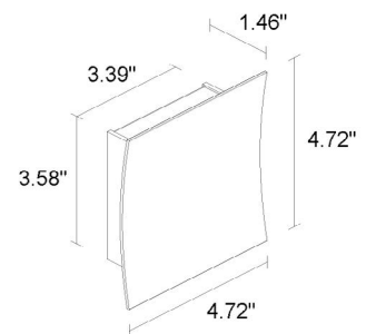
Fixture Dimensions
