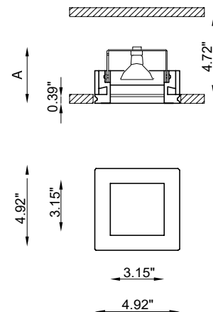
Fixture Dimensions
