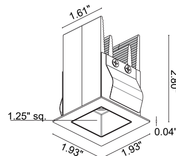
Ceiling Cut-Out: 1.69" x 1.69" Fixture Dimensions
