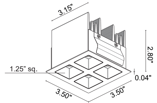
Ceiling Cut-Out: 3.23" x 3.23" Fixture Dimensions
