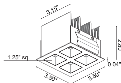
Ceiling Cut-Out: 3.23" x 3.23" Fixture Dimensions
