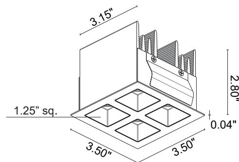
Ceiling Cut-Out: 3.23" x 3.23" Fixture Dimensions
