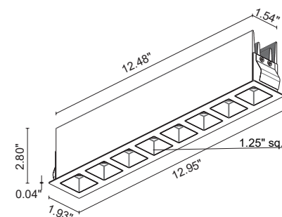
Ceiling Cut-Out: 12.6" x 1.65" Fixture Dimensions
