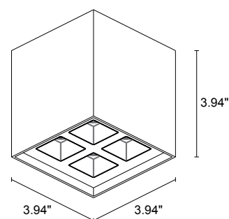
Fixture Dimensions
