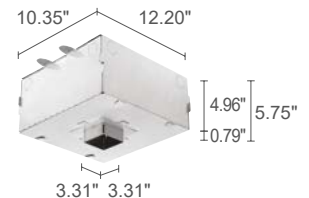
WC8701 Outer casing for rebated installation in solid ceilings (Bitpop 2.2)
