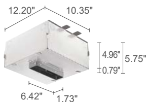
WC8702 Outer casing for rebated installation in solid ceilings (Bitpop 4.1)
