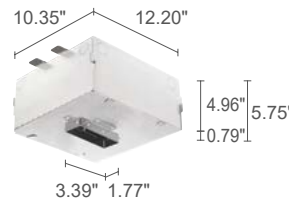
WC8712 Outer casing for rebated installation in solid ceilings (Bitpop 2.1)
