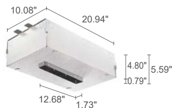
WC8709 Outer casing for rebated installation in solid ceilings (Bitpop 8.1)
