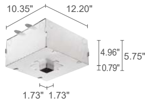
WC8700 Outer casing for rebated installation in solid ceilings (Bitpop 1.0)
