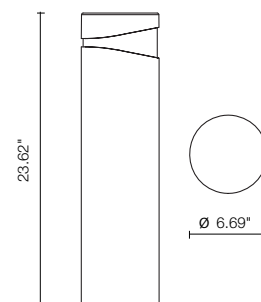
Fixture Dimensions
