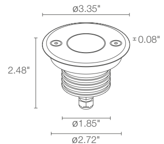
Fixture Dimensions
