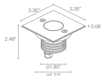
Fixture Dimensions
