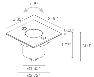
Fixture Dimensions
