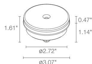
Fixture Dimensions
