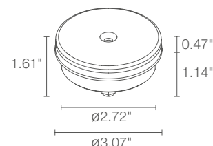
Fixture Dimensions
