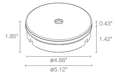
Fixture Dimensions
