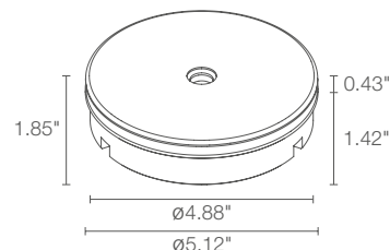
Fixture Dimensions
