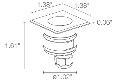
Fixture Dimensions
