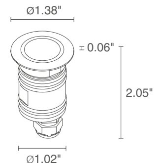
Fixture Dimensions:
