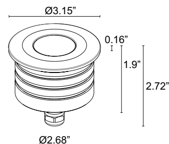
Fixture Dimensions
