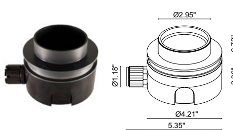
WC5006 Outer Casing 2 ONE REQUIRED
