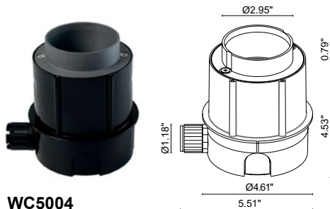
WC5004 Outer Casing 1 ONE REQUIRED
