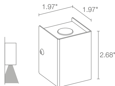
Fixture Dimensions
