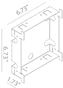
748 01 000 Outer Casing (Housing: Perforated Aluminum)
