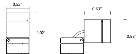
Fixture Dimensions
